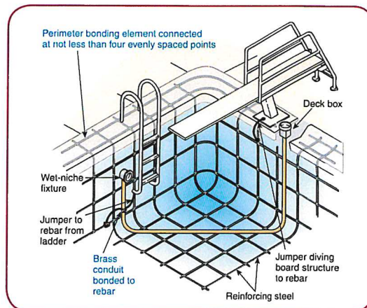
Bonding of conductive metal equipment and parts associated with a swimming pool. Source: National Electrical Code Handbook , Exhibit 680.8, 2011 ed.
