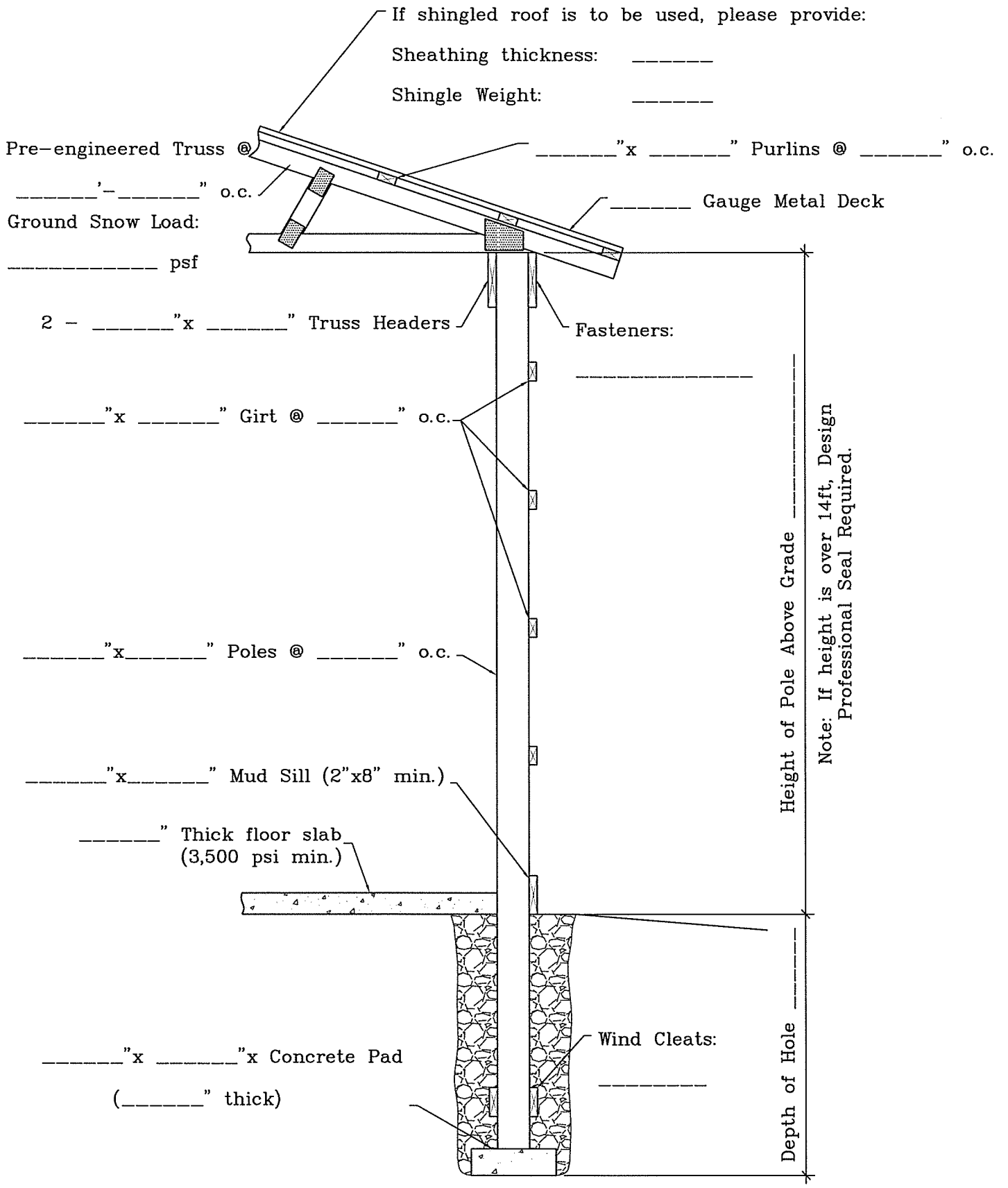
TYPICAL POLE BUILDING
